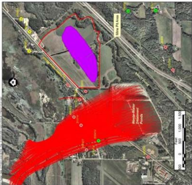
Groundwater Flow Paths from Wastewater Ponds With the Proposed Mine Project
